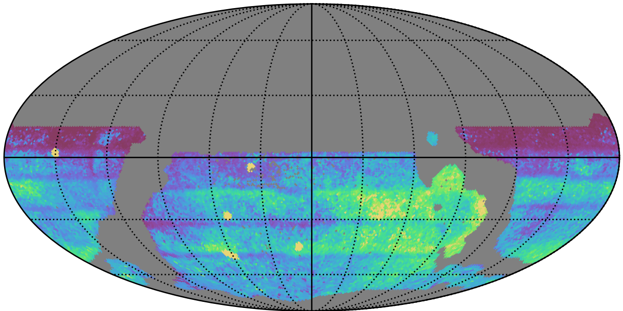
weather_cloudso30v3.4_10yrs WFD all bands: 75th Percentile Intranight Timespan
