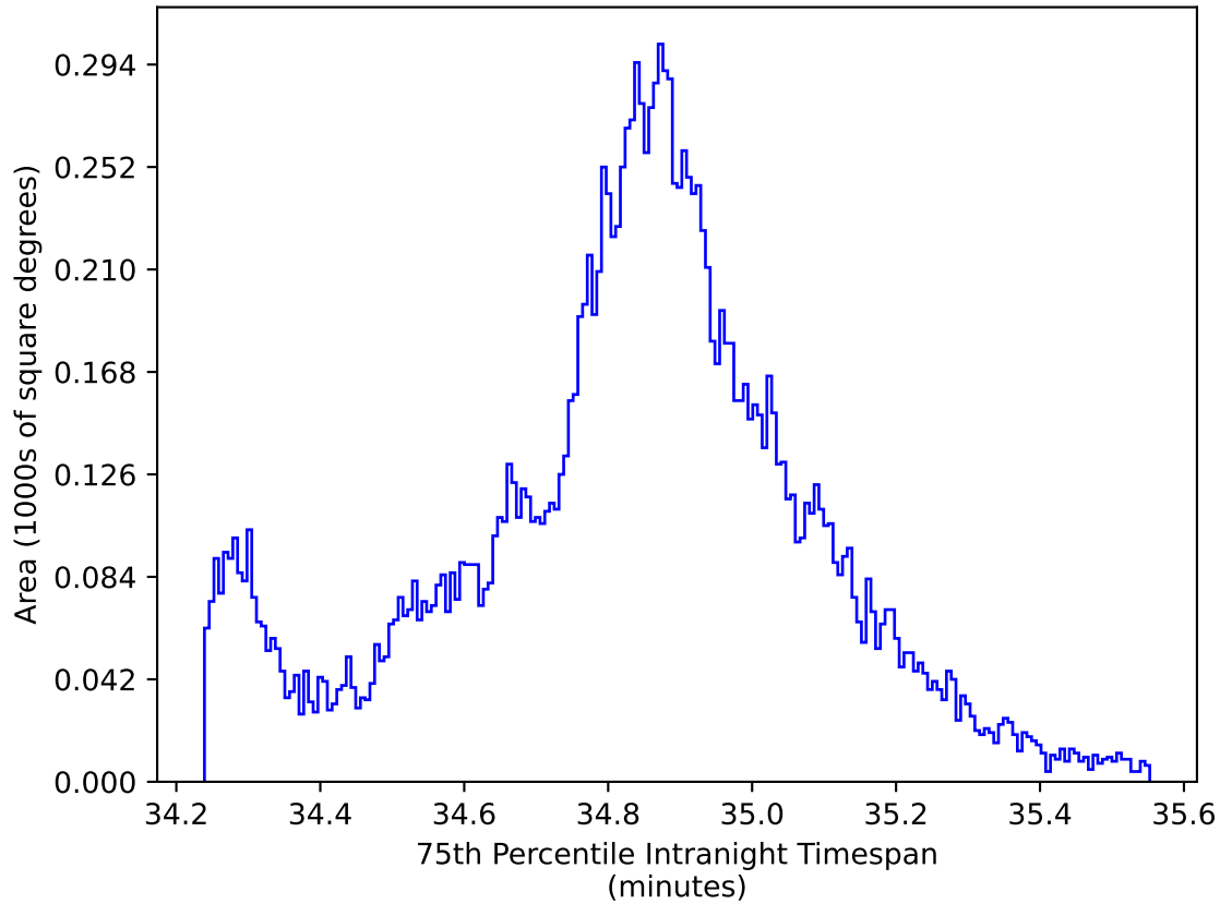
weather_cloudso30v3.4_10yrs WFD all bands: 75th Percentile Intranight Timespan
