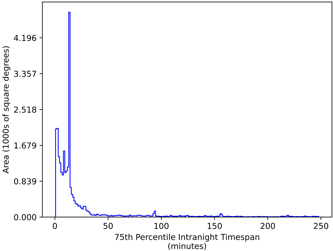
weather_cloudso30v3.4_10yrs All sky z band: 75th Percentile Intranight Timespan
