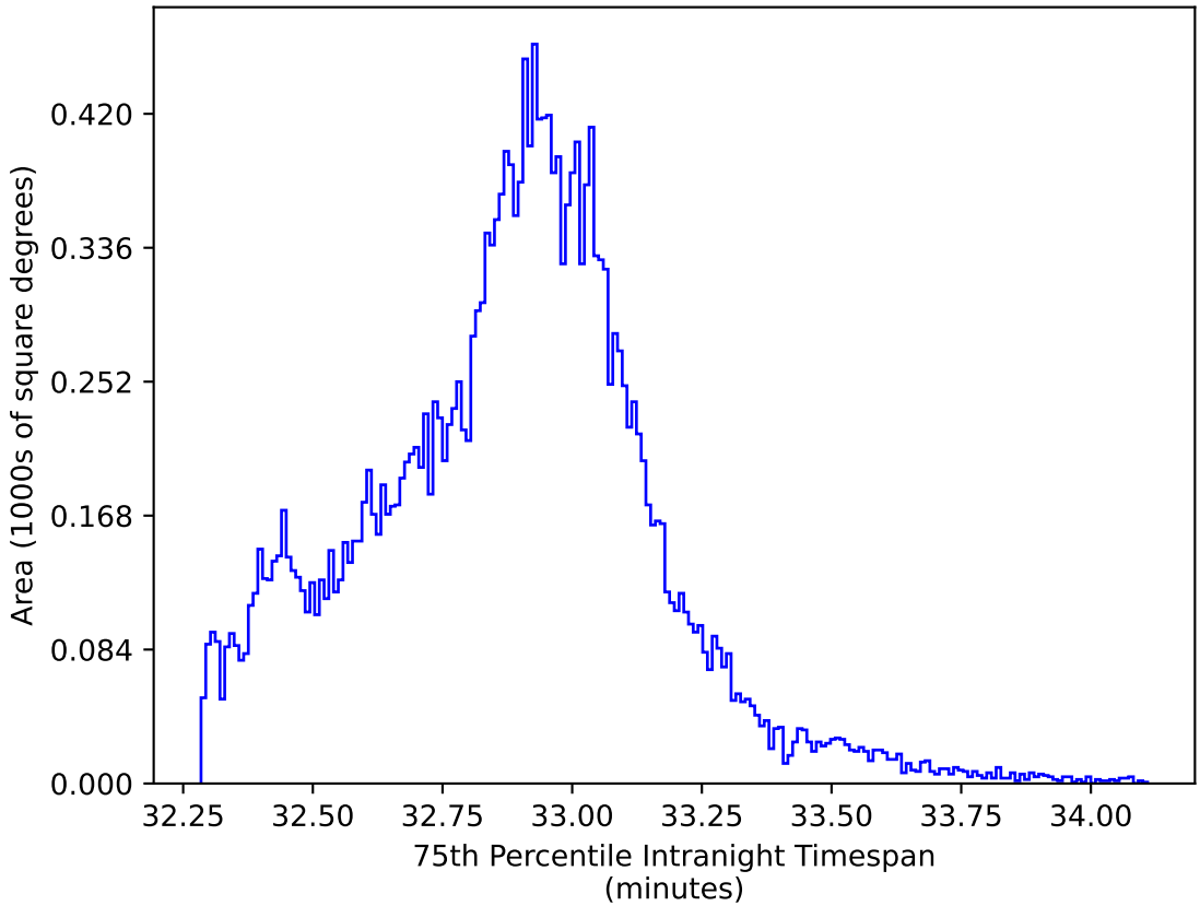
weather_cloudso30v3.4_10yrs All sky y band: 75th Percentile Intranight Timespan
