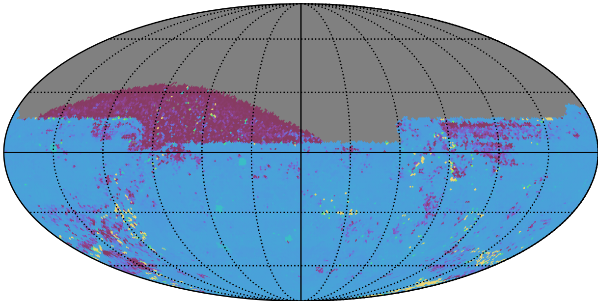
weather_cloudso30v3.4_10yrs All sky ug bands: 75th Percentile Intranight Timespan
