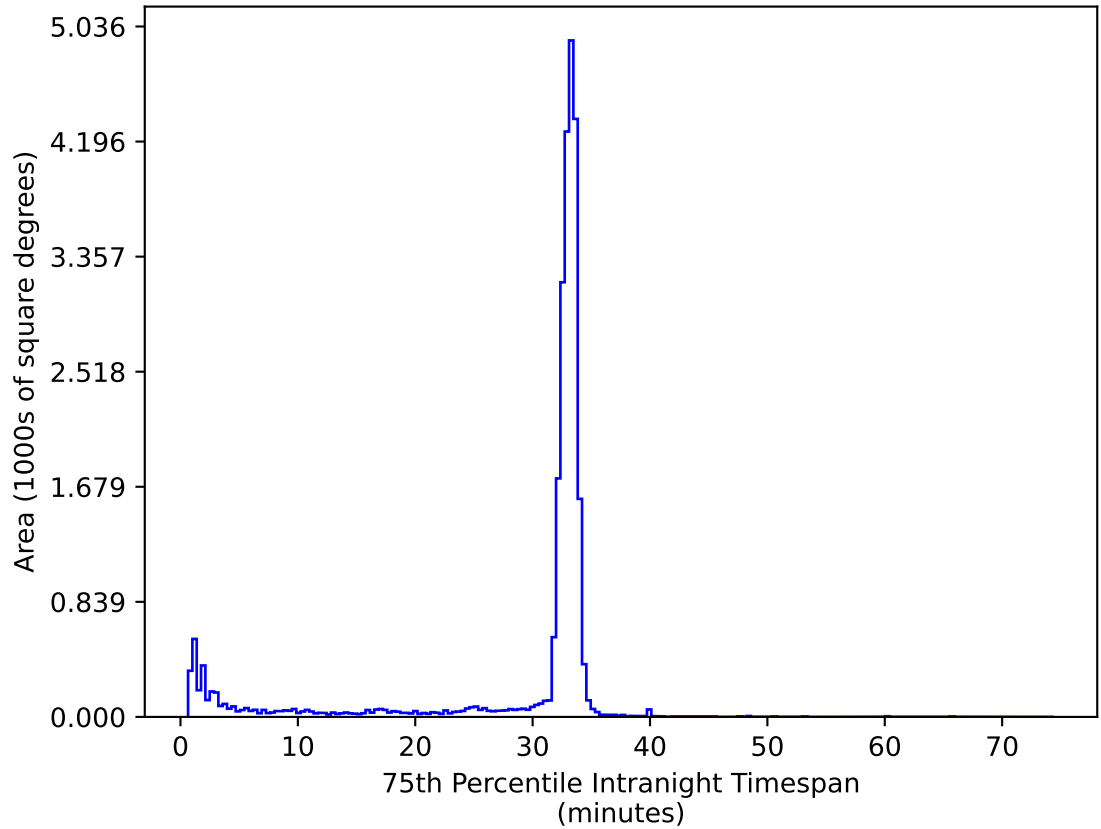
weather_cloudso30v3.4_10yrs All sky ug bands: 75th Percentile Intranight Timespan
