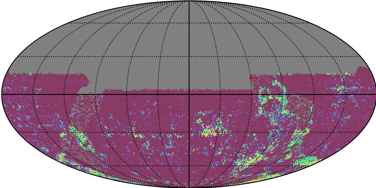
weather_cloudso30v3.4_10yrs All sky u band: 75th Percentile Intranight Timespan
