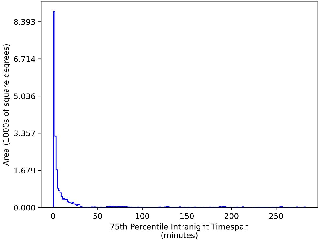
weather_cloudso30v3.4_10yrs All sky u band: 75th Percentile Intranight Timespan
