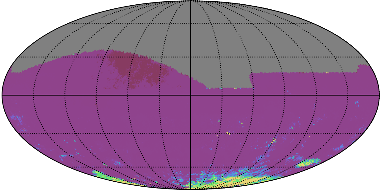
weather_cloudso30v3.4_10yrs All sky ri bands: 75th Percentile Intranight Timespan
