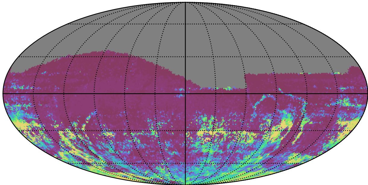
weather_cloudso30v3.4_10yrs All sky r band: 75th Percentile Intranight Timespan
