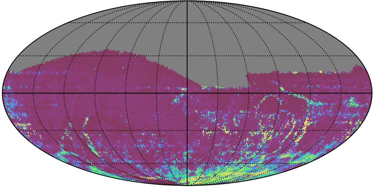
weather_cloudso30v3.4_10yrs All sky i band: 75th Percentile Intranight Timespan
