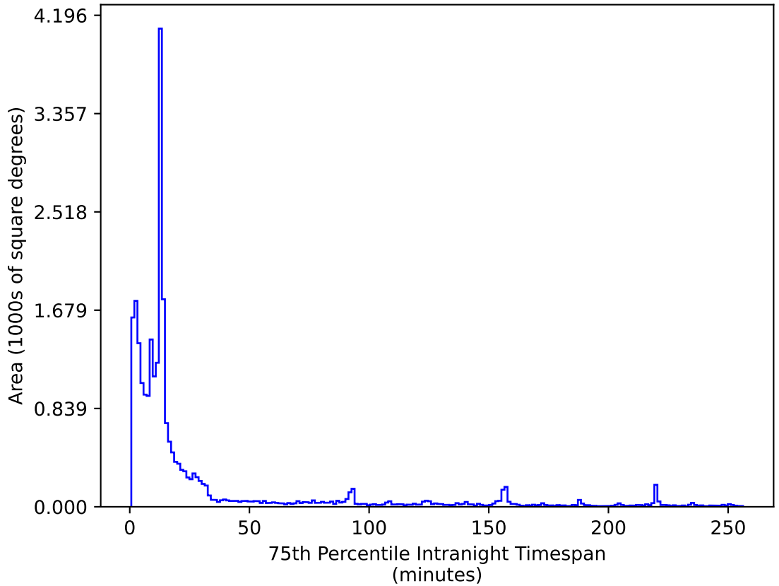
weather_cloudso30v3.4_10yrs All sky i band: 75th Percentile Intranight Timespan
