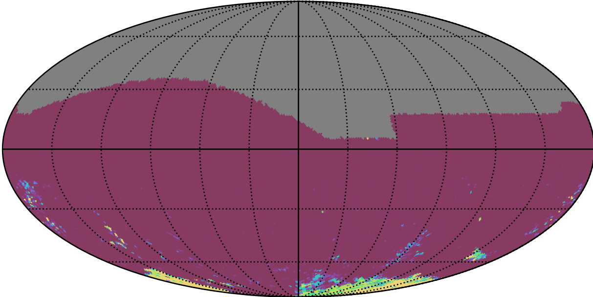
weather_cloudso30v3.4_10yrs All sky gr bands: 75th Percentile Intranight Timespan
