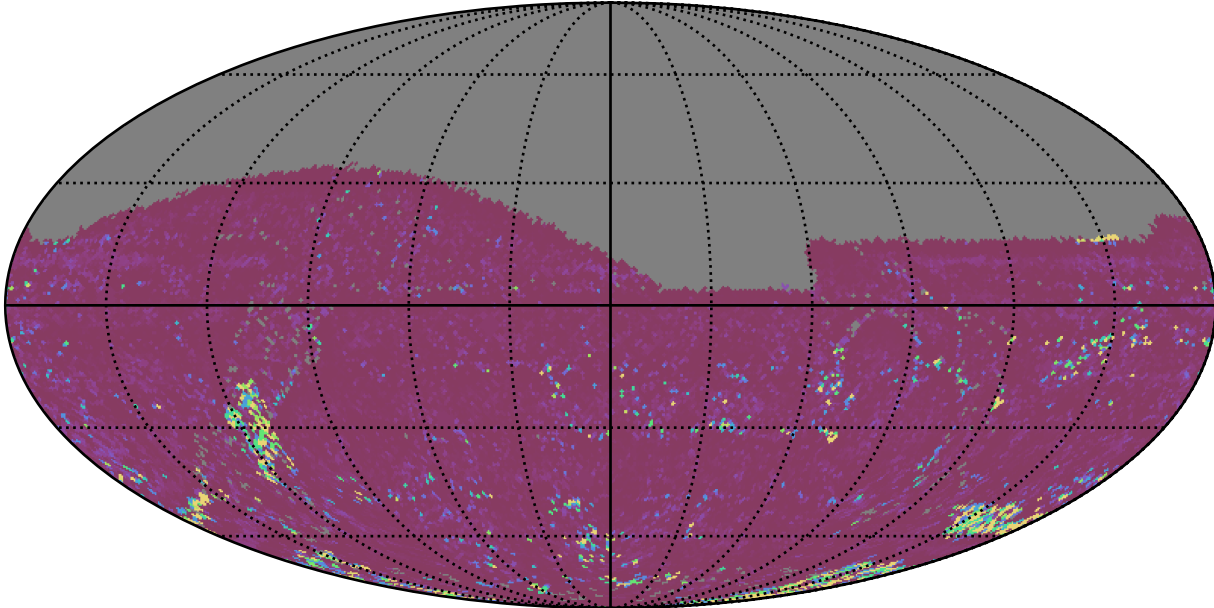
weather_cloudso30v3.4_10yrs All sky g band: 75th Percentile Intranight Timespan
