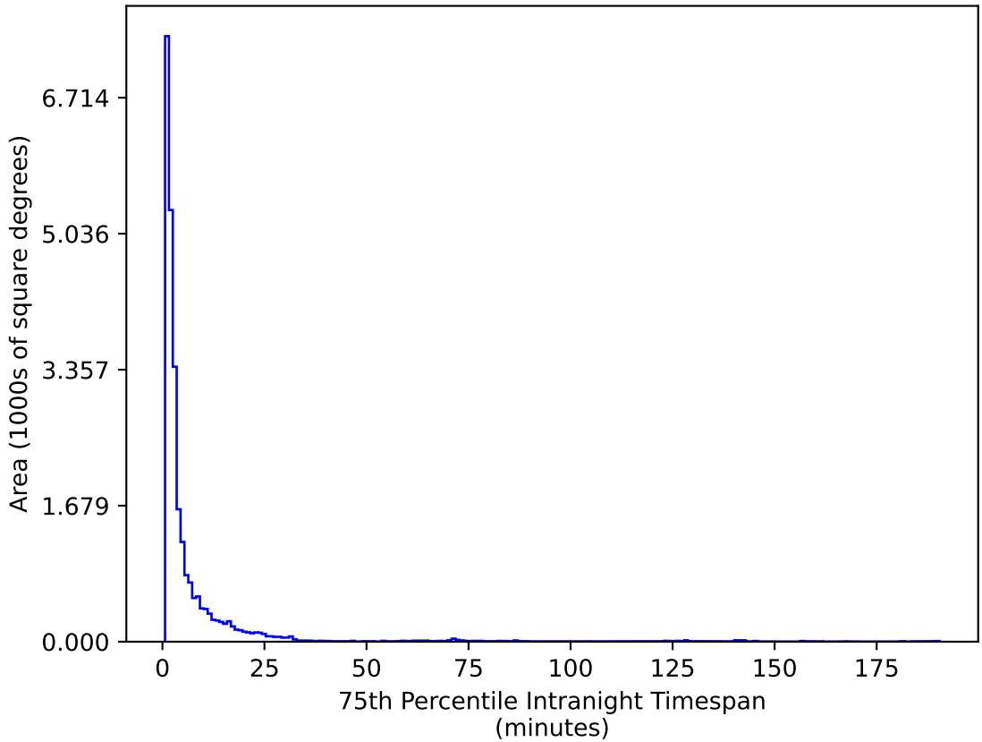
weather_cloudso30v3.4_10yrs All sky g band: 75th Percentile Intranight Timespan
