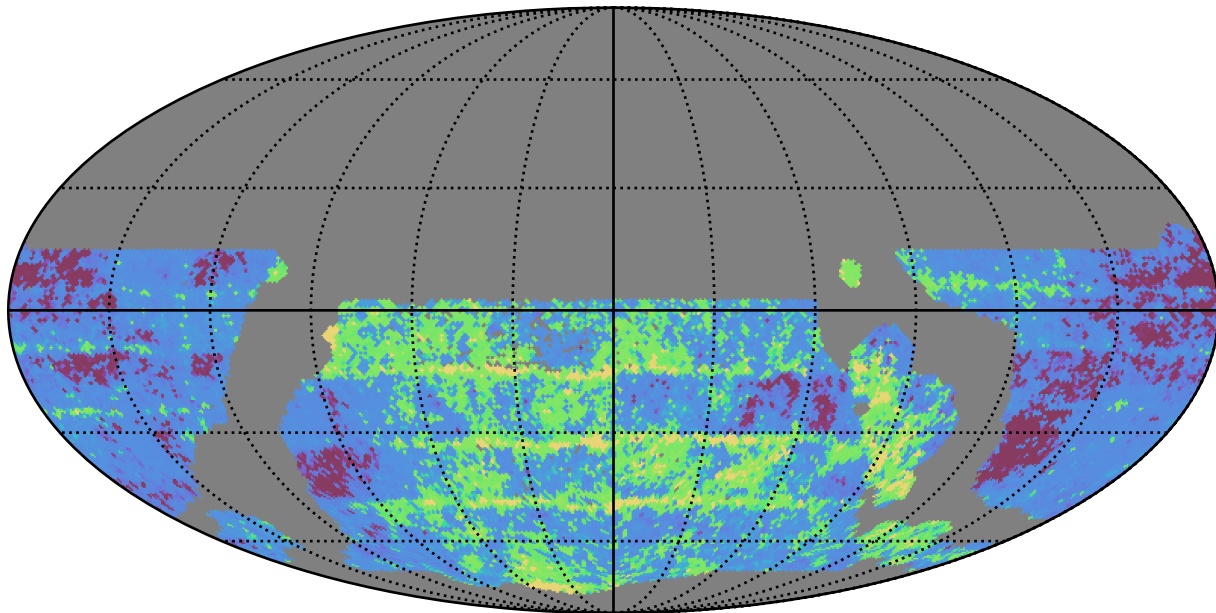
weather_cloudso30v3.4_10yrs WFD z band: 20thPercentile Inter-Night Gap
