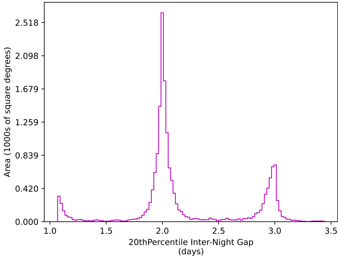
weather_cloudso30v3.4_10yrs WFD z band: 20thPercentile Inter-Night Gap
