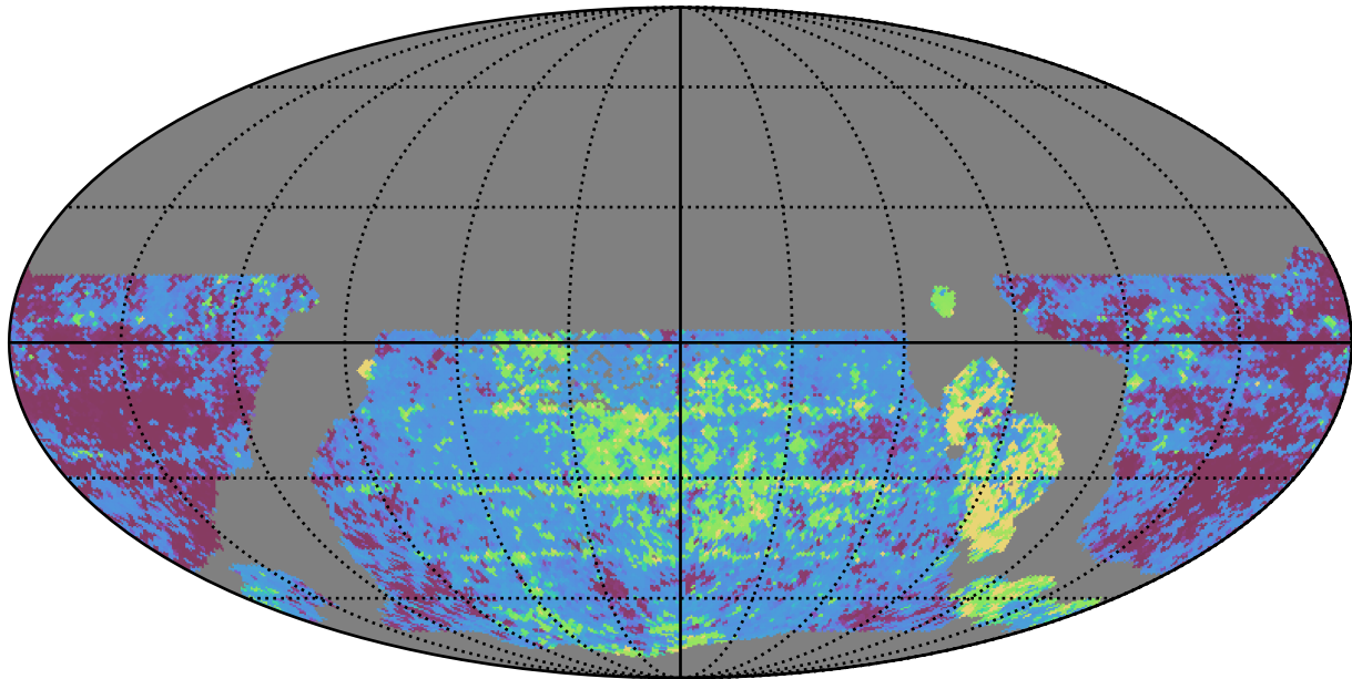
weather_cloudso30v3.4_10yrs WFD y band: 20thPercentile Inter-Night Gap
