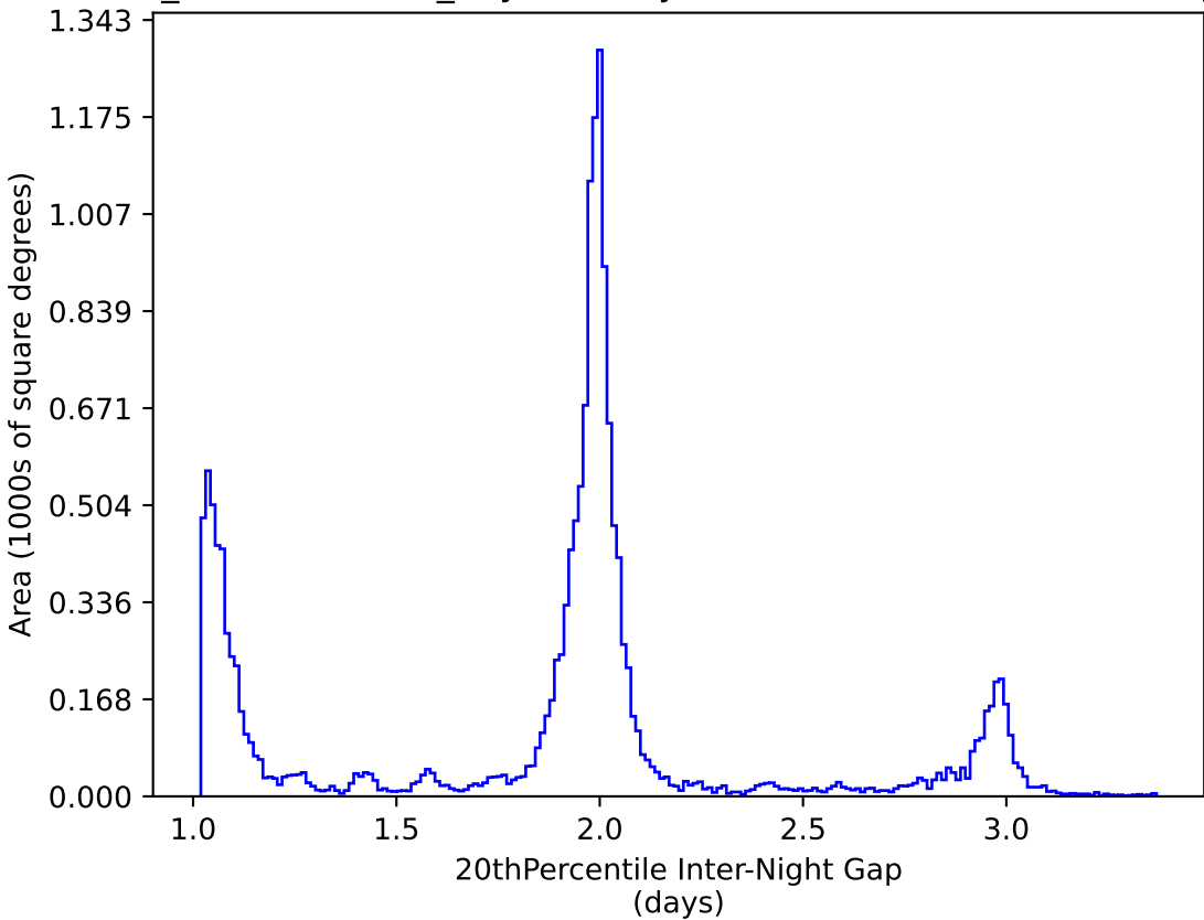
weather_cloudso30v3.4_10yrs WFD y band: 20thPercentile Inter-Night Gap
