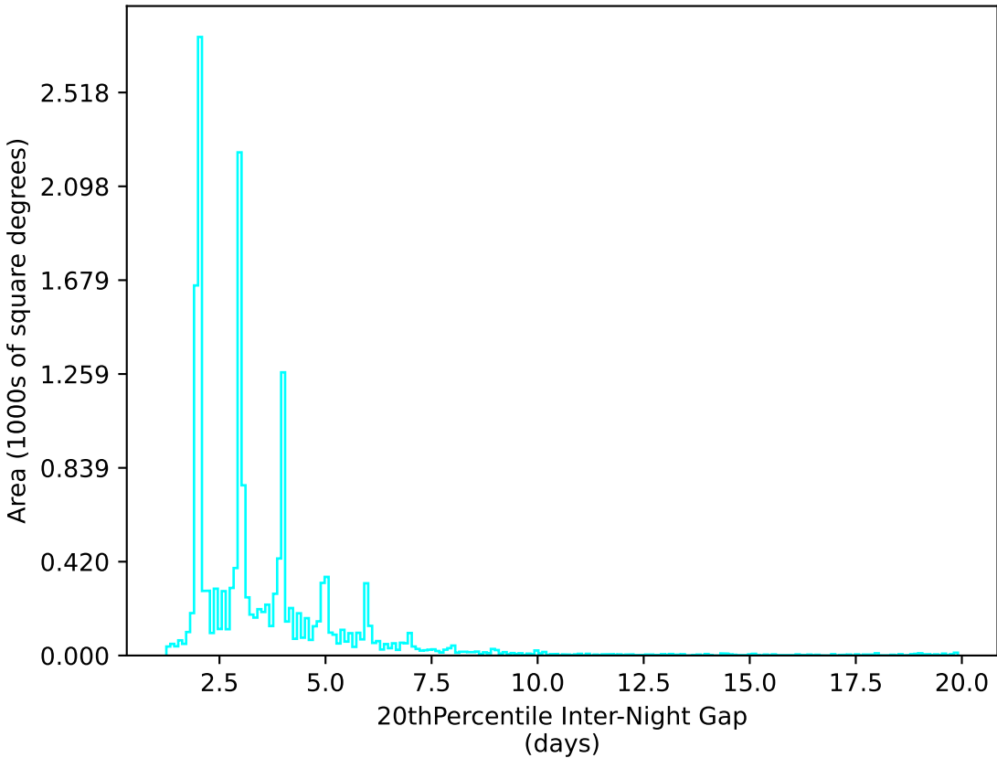
weather_cloudso30v3.4_10yrs WFD u band: 20thPercentile Inter-Night Gap
