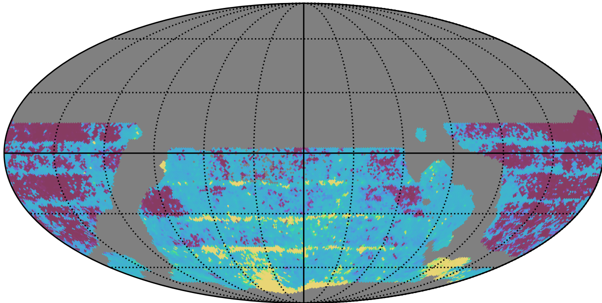
weather_cloudso30v3.4_10yrs WFD r band: 20thPercentile Inter-Night Gap
