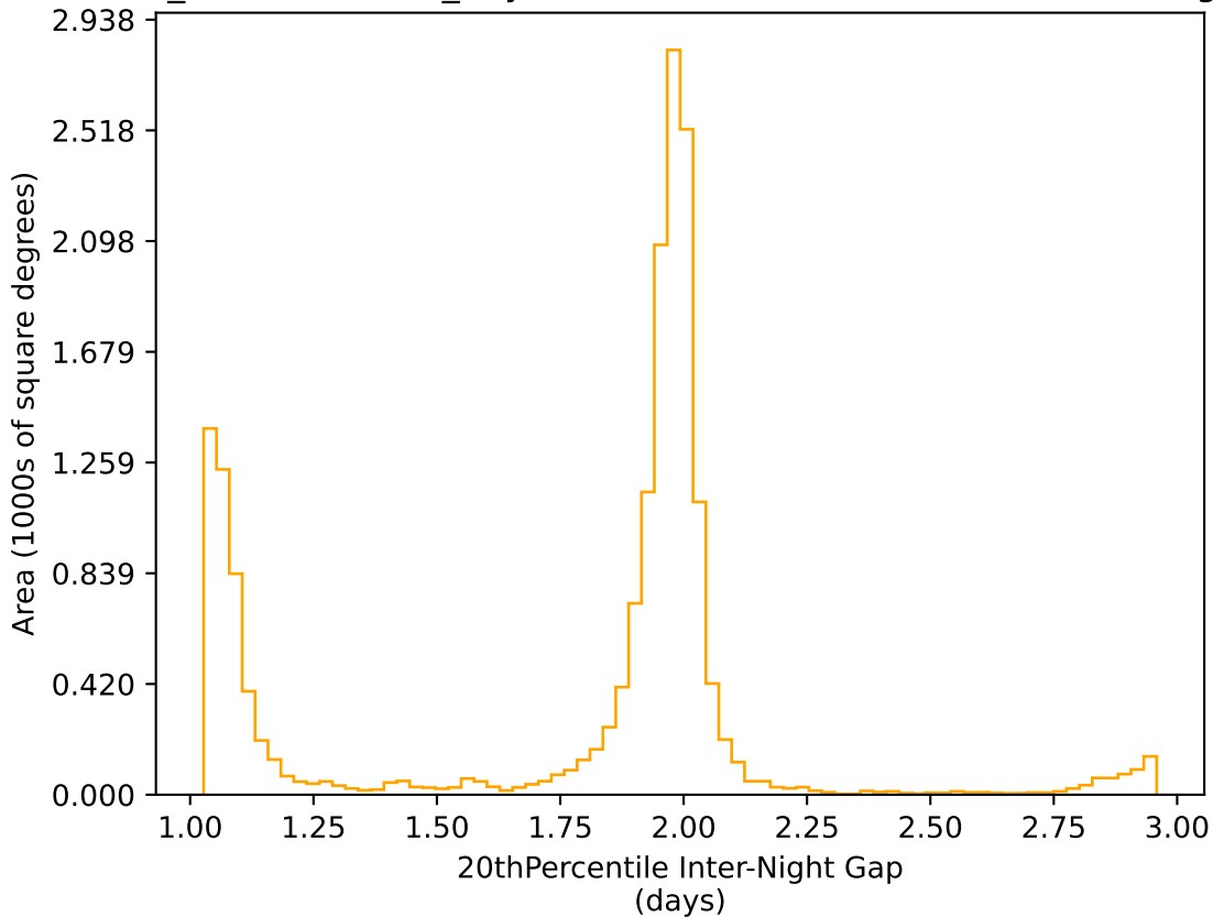
weather_cloudso30v3.4_10yrs WFD r band: 20thPercentile Inter-Night Gap
