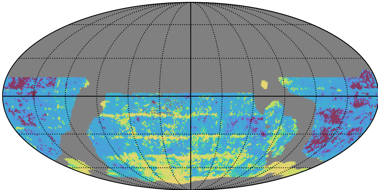
weather_cloudso30v3.4_10yrs WFD i band: 20thPercentile Inter-Night Gap
