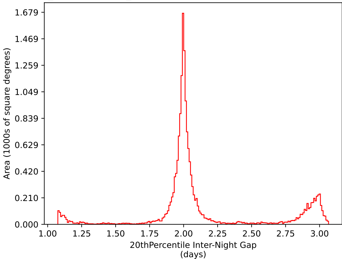
weather_cloudso30v3.4_10yrs WFD i band: 20thPercentile Inter-Night Gap
