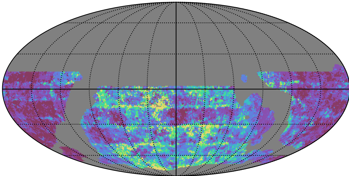
weather_cloudso30v3.4_10yrs WFD g band: 20thPercentile Inter-Night Gap
