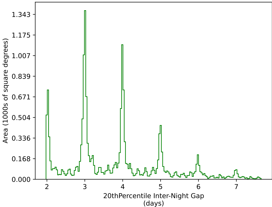
weather_cloudso30v3.4_10yrs WFD g band: 20thPercentile Inter-Night Gap
