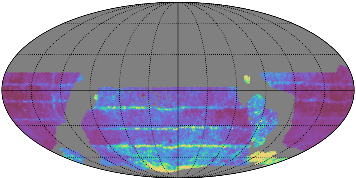
weather_cloudso30v3.4_10yrs WFD all bands: 20thPercentile Inter-Night Gap
