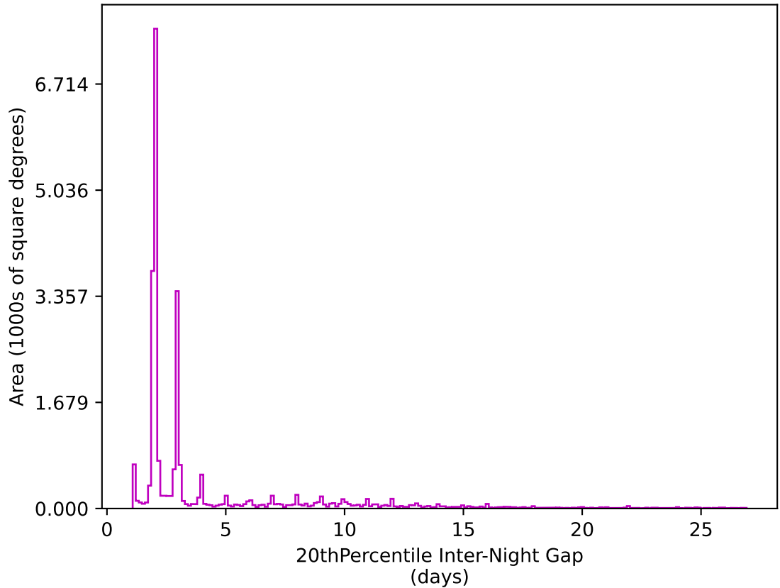
weather_cloudso30v3.4_10yrs All sky z band: 20thPercentile Inter-Night Gap
