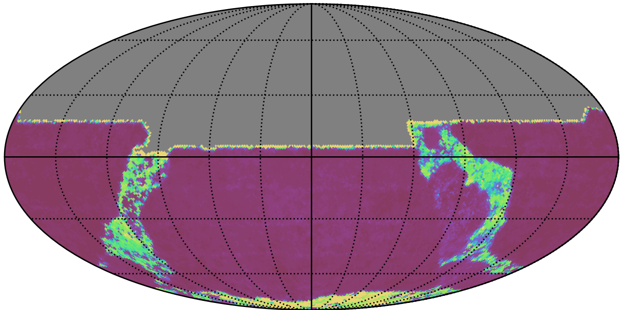
weather_cloudso30v3.4_10yrs All sky y band: 20thPercentile Inter-Night Gap
