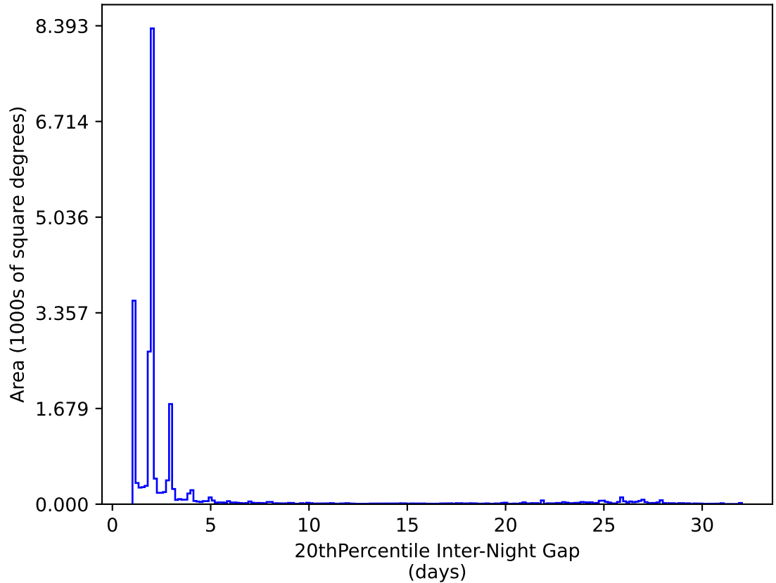
weather_cloudso30v3.4_10yrs All sky y band: 20thPercentile Inter-Night Gap
