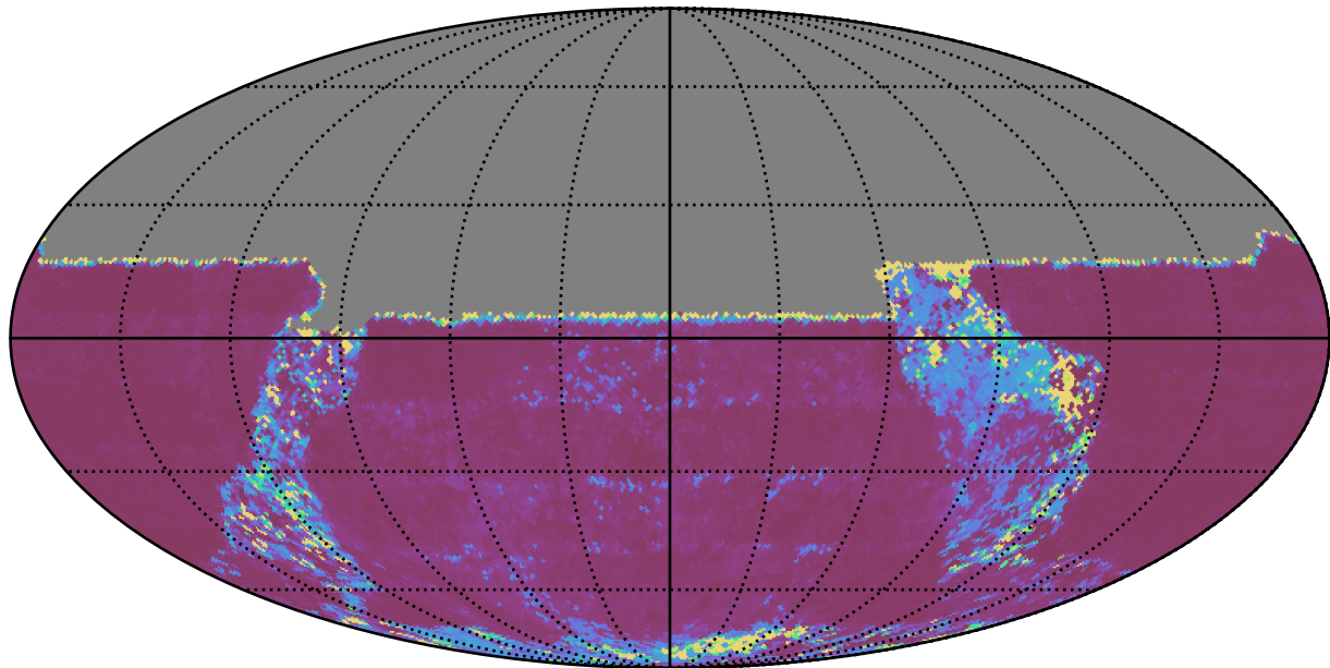
weather_cloudso30v3.4_10yrs All sky u band: 20thPercentile Inter-Night Gap
