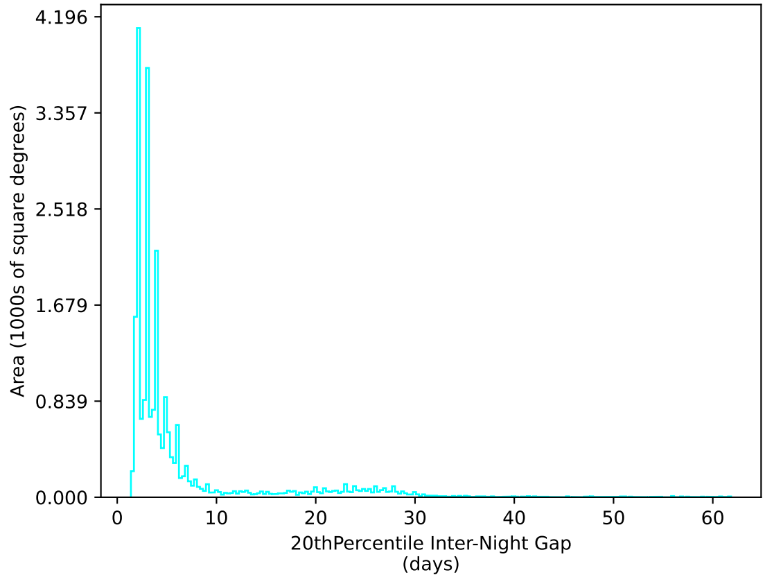
weather_cloudso30v3.4_10yrs All sky u band: 20thPercentile Inter-Night Gap
