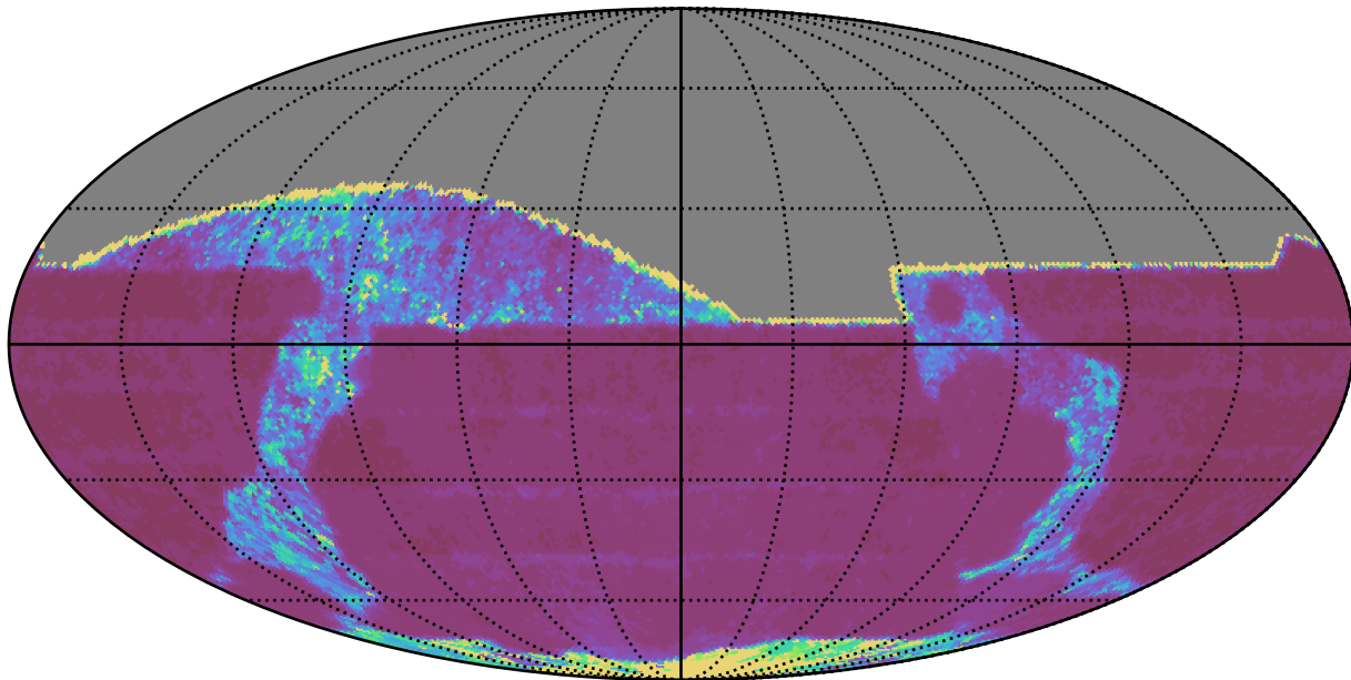
weather_cloudso30v3.4_10yrs All sky r band: 20thPercentile Inter-Night Gap
