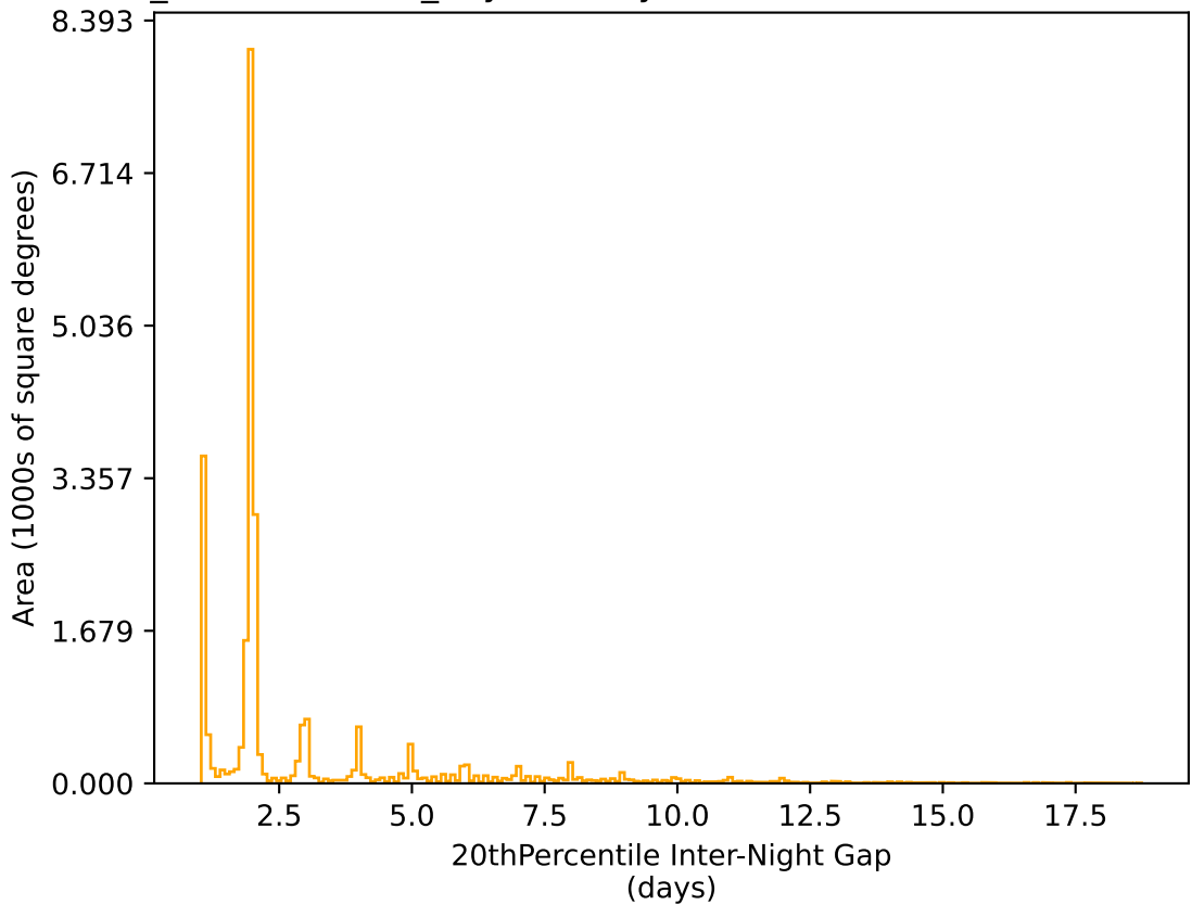
weather_cloudso30v3.4_10yrs All sky r band: 20thPercentile Inter-Night Gap
