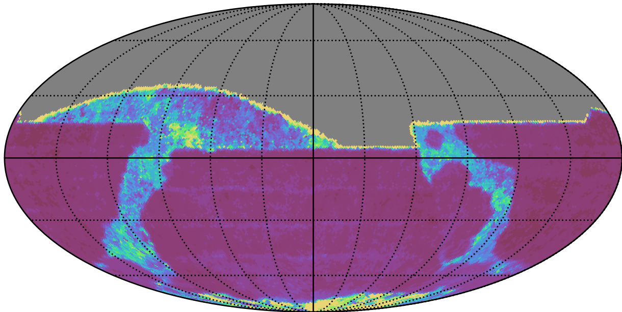
weather_cloudso30v3.4_10yrs All sky i band: 20thPercentile Inter-Night Gap
