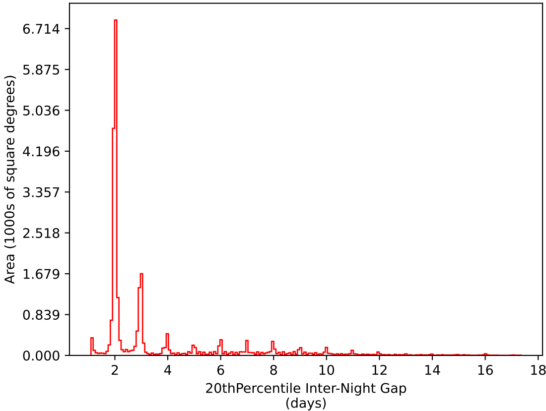
weather_cloudso30v3.4_10yrs All sky i band: 20thPercentile Inter-Night Gap
