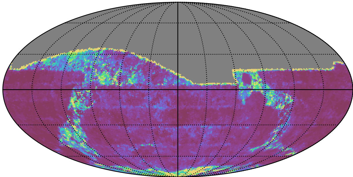
weather_cloudso30v3.4_10yrs All sky g band: 20thPercentile Inter-Night Gap
