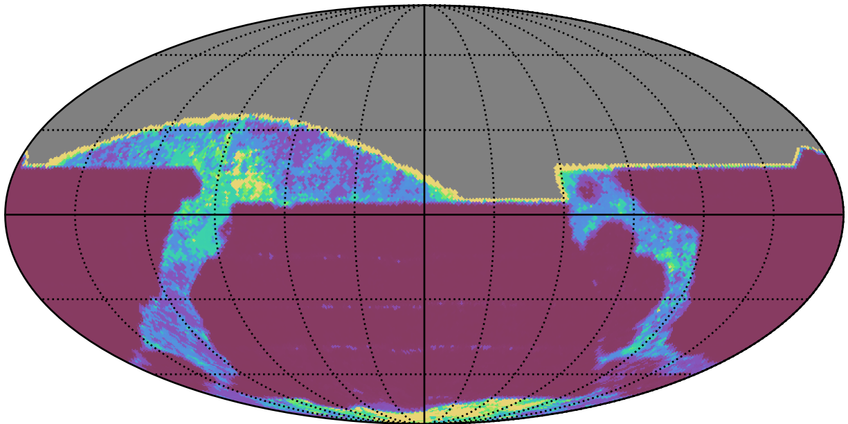
weather_cloudso30v3.4_10yrs All sky all bands: 20thPercentile Inter-Night Gap
