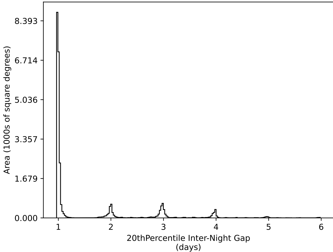
weather_cloudso30v3.4_10yrs All sky all bands: 20thPercentile Inter-Night Gap
