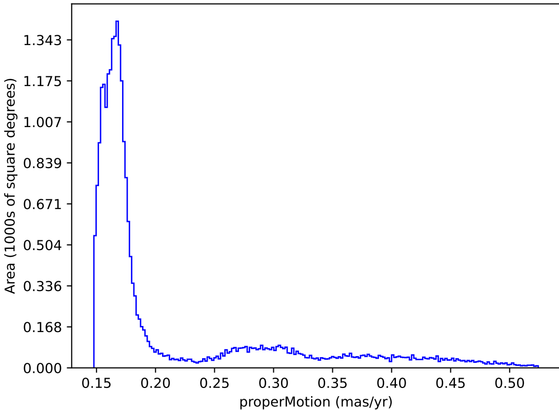
weather_cloudso30v3.4_10yrs : properMotion
