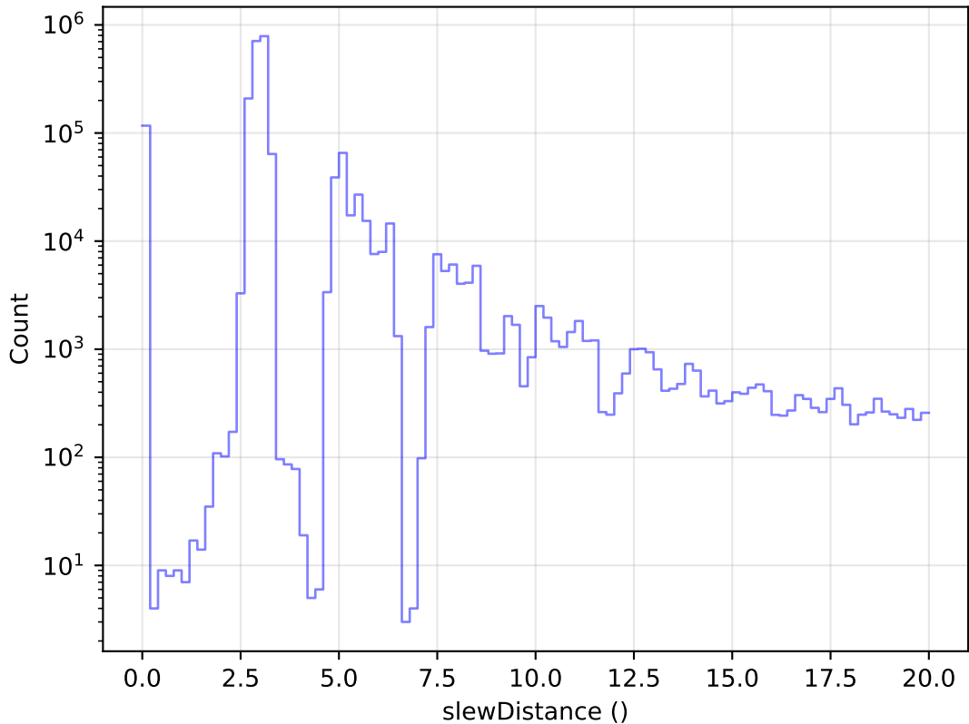
weather_cloudso30v3.4_10yrs All visits: Zoom Slew Distance Histogram
