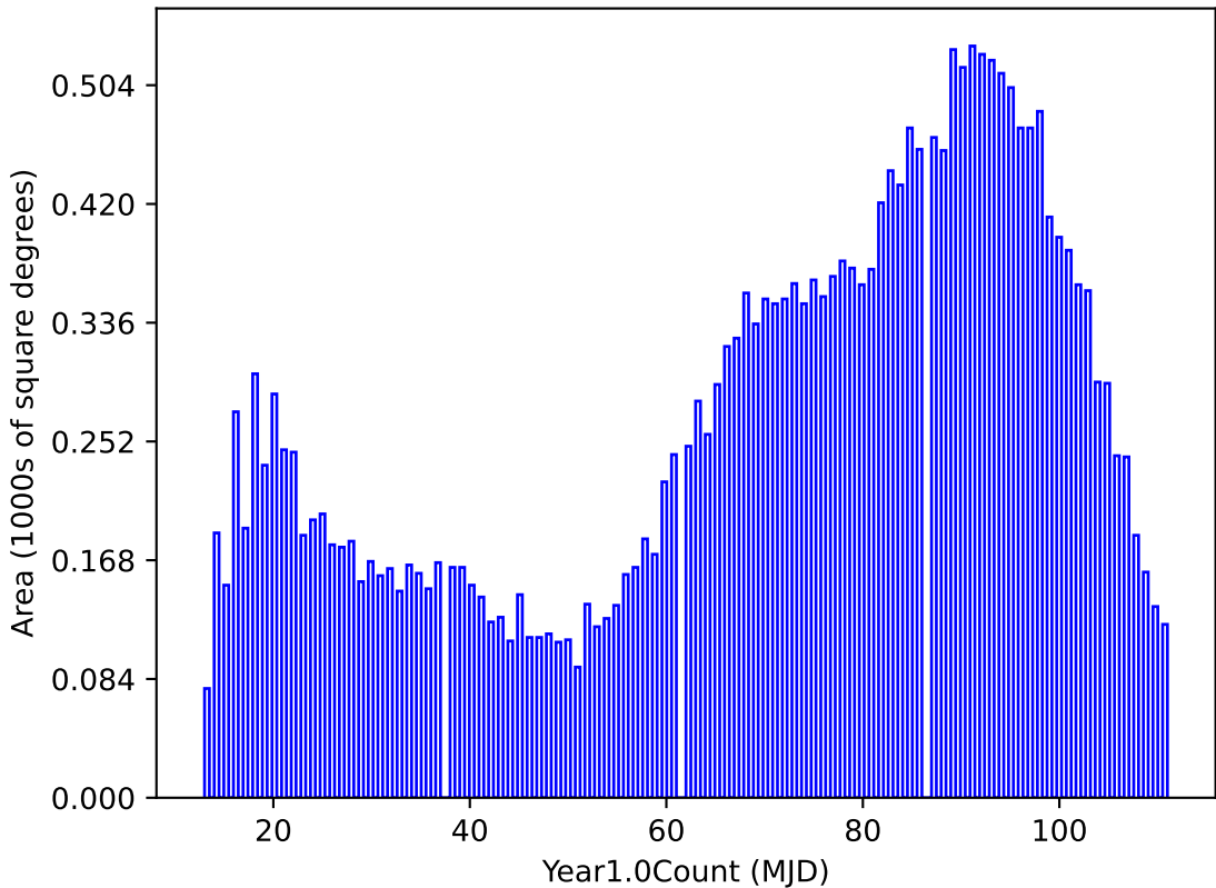
weather_cloudso30v3.4_10yrs night < 365.25: Year1.0Count
