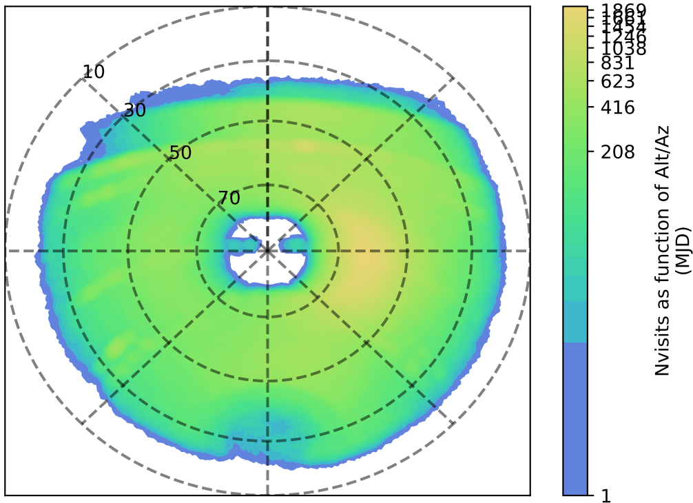
weather_cloudso30v3.4_10yrs y: Nvisits as function of Alt/Az
