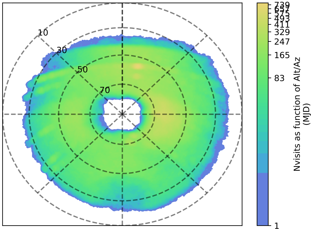
weather_cloudso30v3.4_10yrs u: Nvisits as function of Alt/Az
