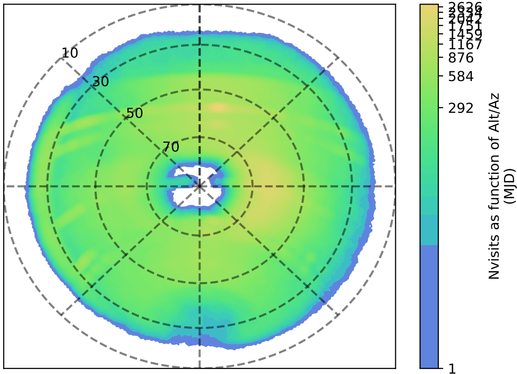
weather_cloudso30v3.4_10yrs r: Nvisits as function of Alt/Az
