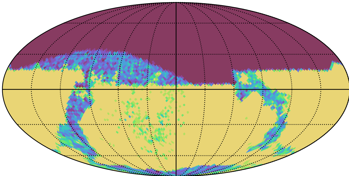
weather_cloudso30v3.4_10yrs z and night < 365: N year 1
