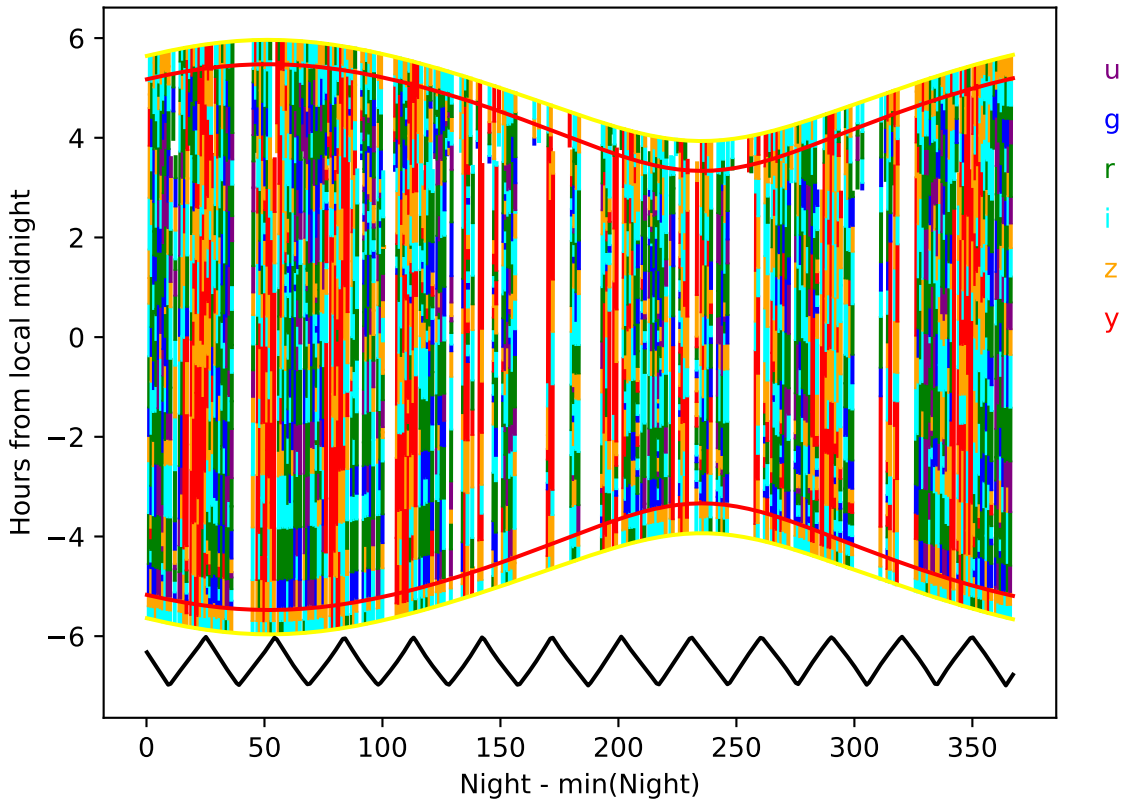
weather_cloudso30v3.4_10yrs year 7-8: Hourglass
