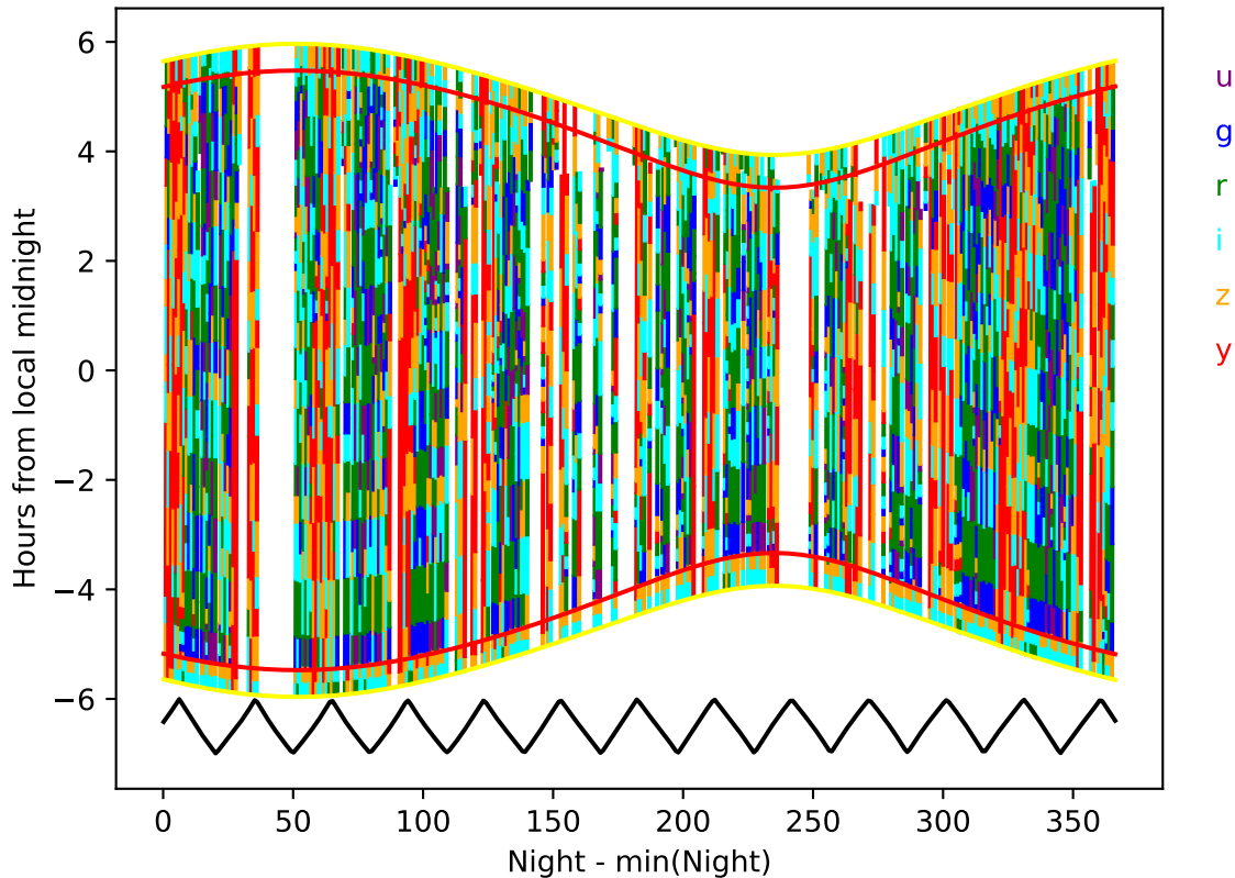
weather_cloudso30v3.4_10yrs year 6-7: Hourglass
