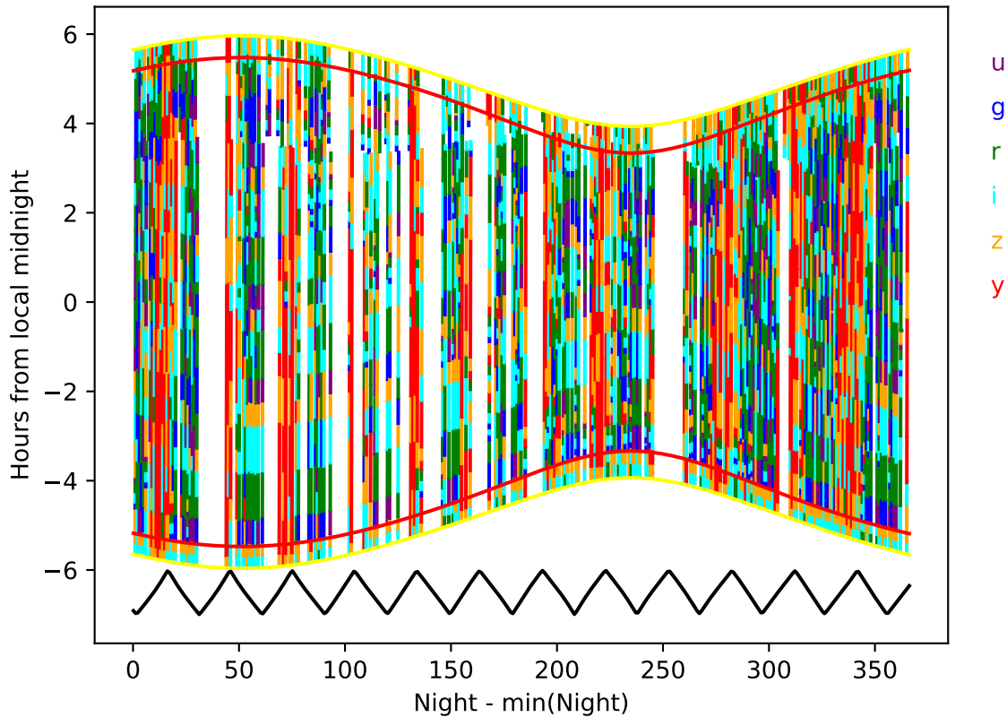
weather_cloudso30v3.4_10yrs year 5-6: Hourglass
