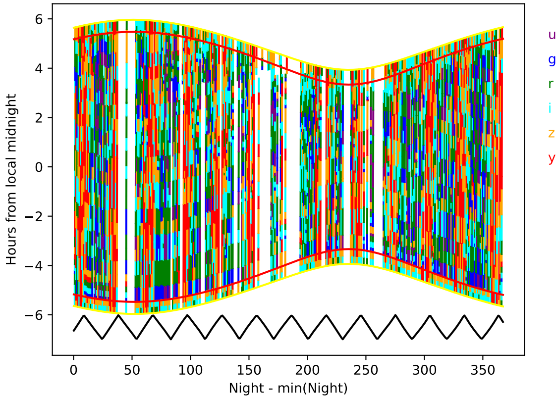
weather_cloudso30v3.4_10yrs year 3-4: Hourglass
